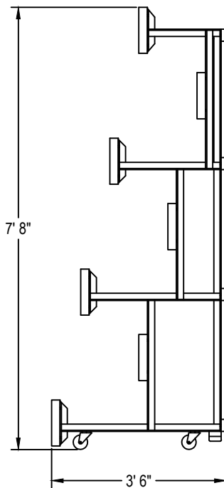
STORAGE POSITION
