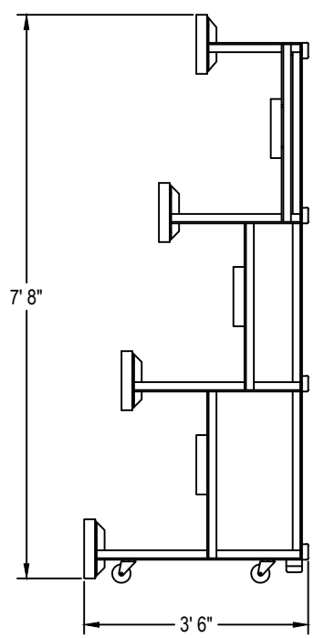
STORAGE POSITION
