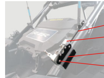
"A" support Locking system "A1" support 1/4" x 1 1/2" screws
