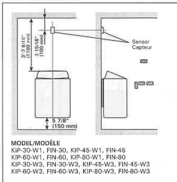
Figure 8. The place of the temperature sensor of the control unit in connection with wall-mounted heaters
