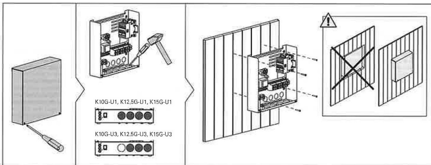
Figure 5. Opening the power unit cover and mounting the unit to a wall Figure 5. Ouverture du cache du bloc d'alimentations et fixations murales
