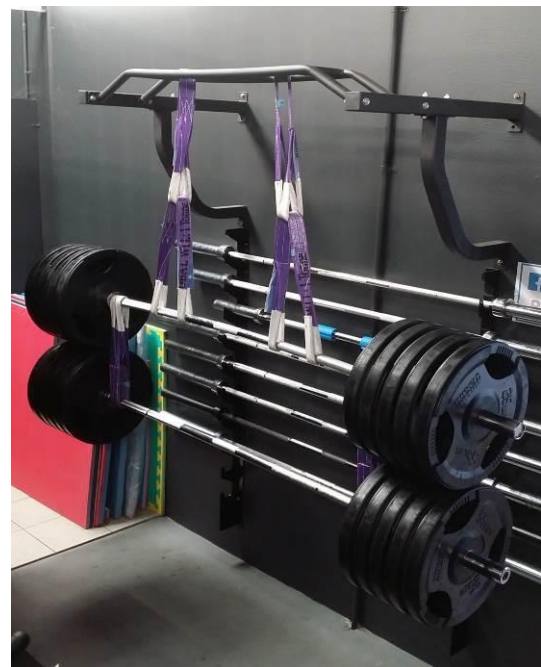
Figure: 2 Subject: View of the multi grip chin up bar with the distributed test load applied.
