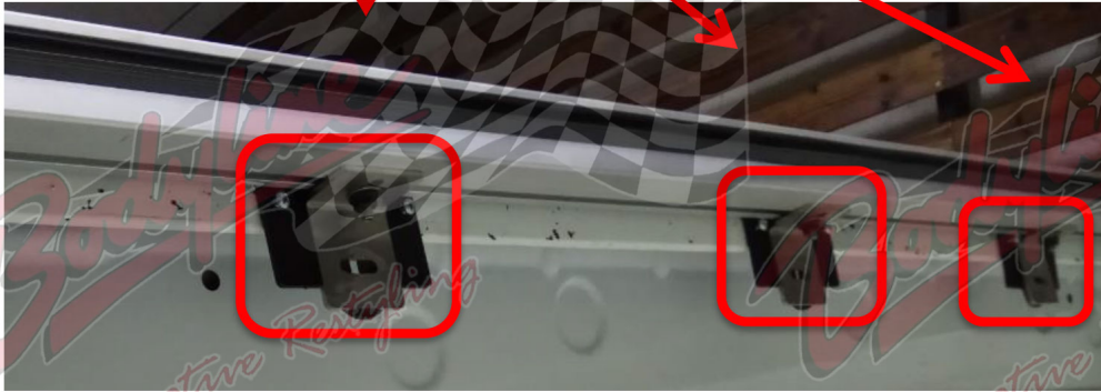
11. Fixing the brackets with ① D6 washer, M6 nut. 3 sets on each side track.
