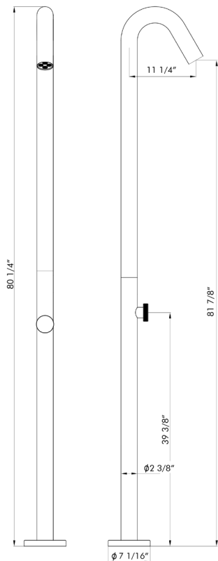
Specs drawing.
