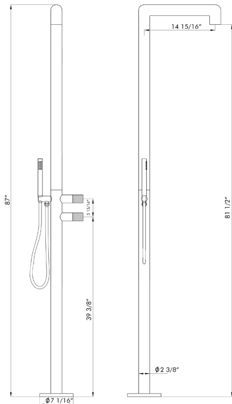
Specs drawing.
