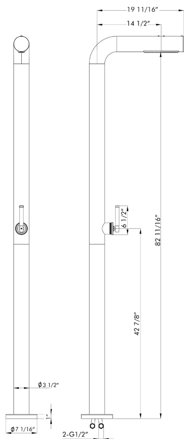
Specs drawing.
