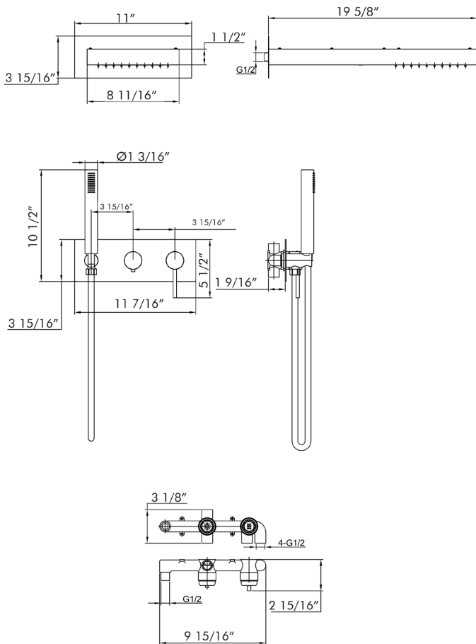
Specs drawing.
