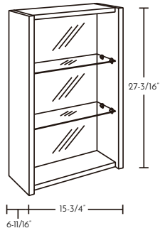
16" SMALL OPEN CABINET
