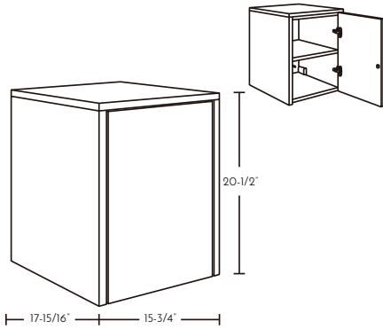
16" LOWER SIDE CABINET
