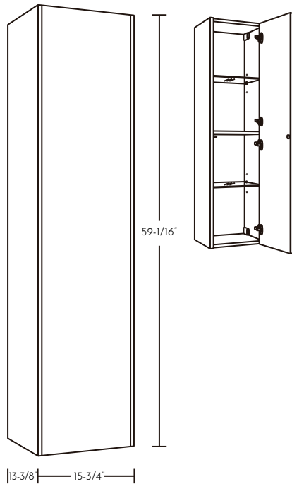
16" TALL SIDE CABINET
