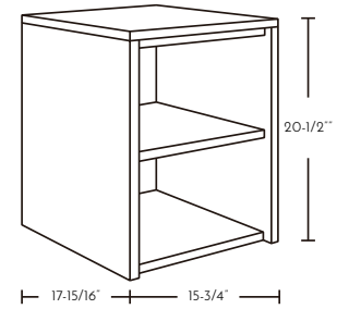
16" LOWER OPEN SIDE CABINET
