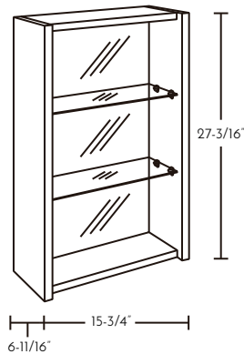
16" SMALL OPEN CABINET
