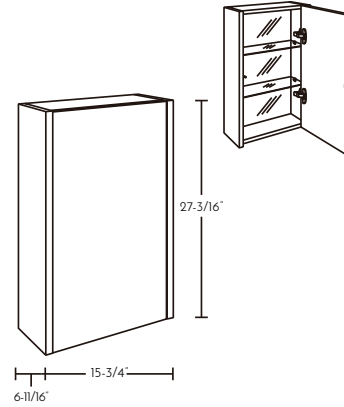
16" SMALL SIDE CABINET
