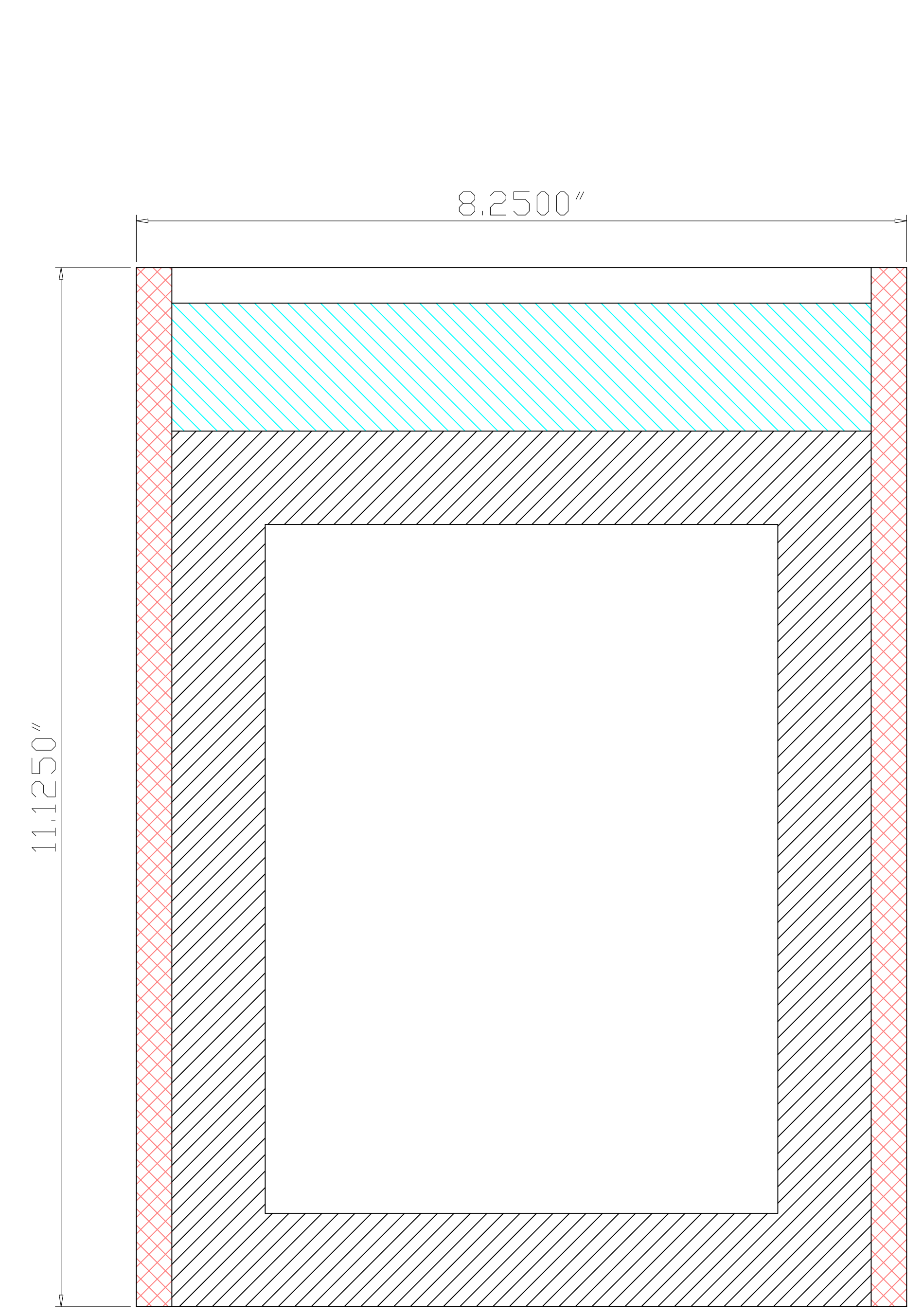
FINISHED POUCH FRONT
