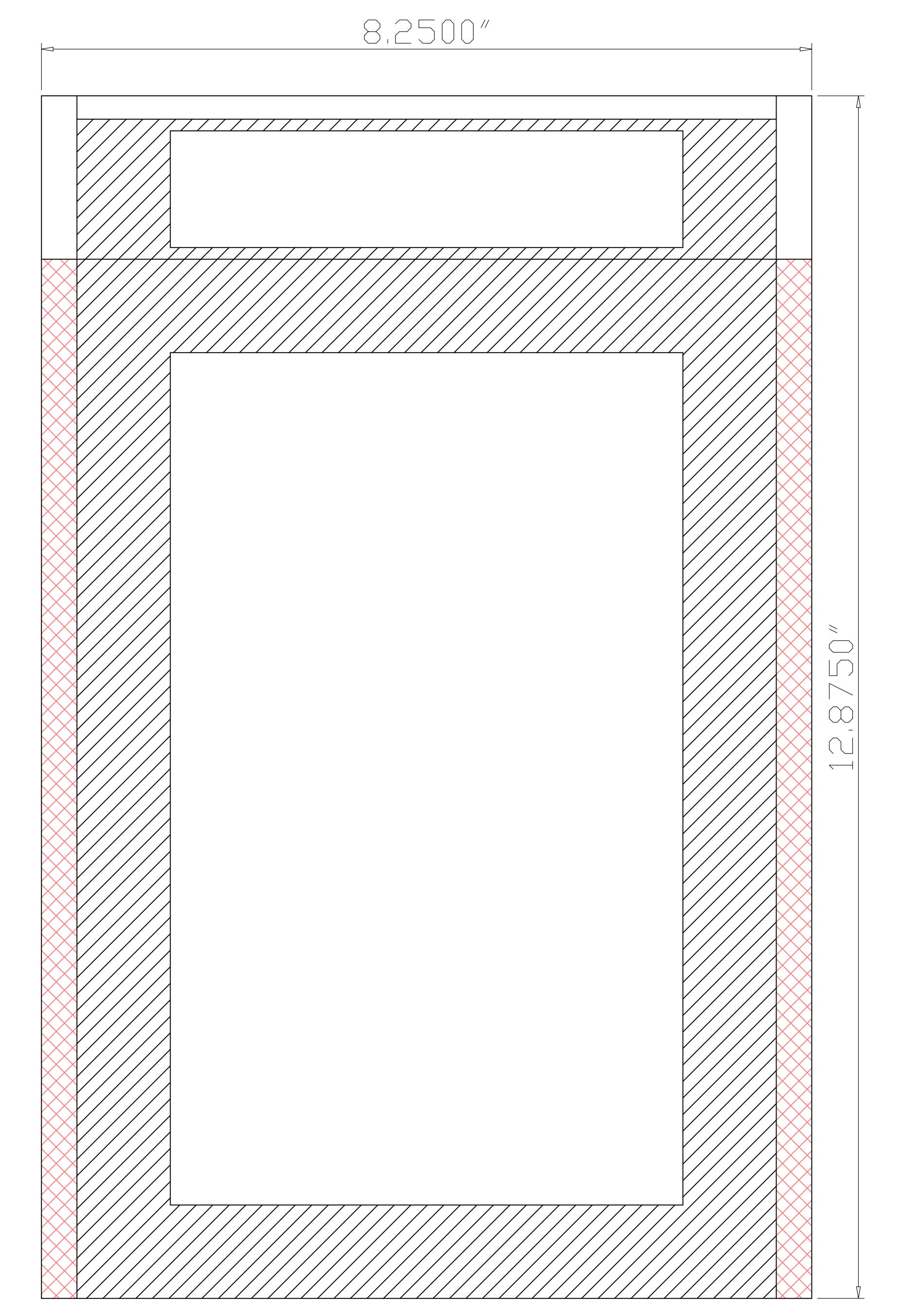
FINISHED POUCH BACK
