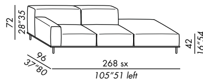
terminale penisola / peninsula end unit 270
