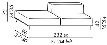
elemento penisola / peninsula unit 235
