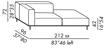
angolo penisola / peninsula corner unit 215
