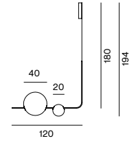
SUPERB-ALL HORIZONTAL L 120 Ø40-Ø30
