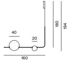
SUPERB-ALL HORIZONTAL L 160 Ø40-Ø30
