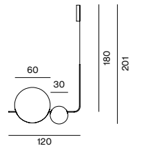
SUPERB-ALL HORIZONTAL L 120 Ø60-Ø30
