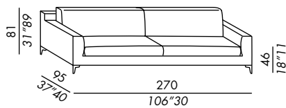
sofa 270
