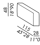
bracciolo / armrest DEEP LARGE 48
