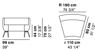
cod. 1186 / closed element 30° R190
