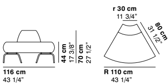
cod. 1185 / open element 60° R110
