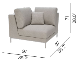
Corner seat
