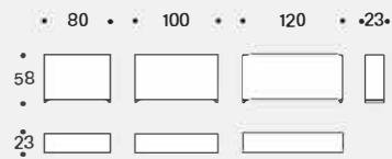
Schienali / Backrests / 23
