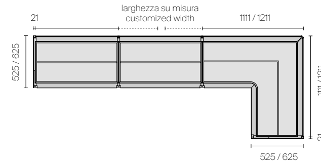
Composizione ad angolo Cover Open Composition with internal corner Cover Open
