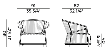
923/PL lounge \ lounge armchair
