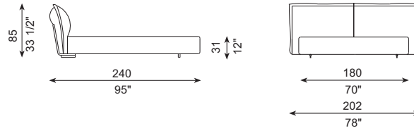
REF. 489-CM4 Colchón - Mattress 160 cm x 200 cm
