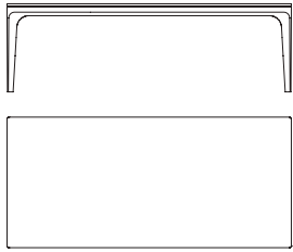
70275 Tavolo rettangolare in acero, top marmo Rectangular table in maple wood, marble top cm 210 x 100 x h 74 in 82 3/4 x 43 3/8 x h 29 1/8
