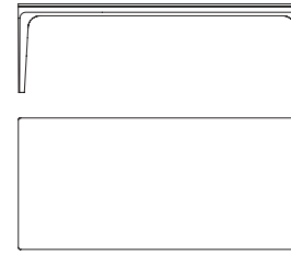
70255 Tavolo rettangolare in acero, top marmo Rectangular table in maple wood, marble top cm 240 x 110 x h 74 in 94 1/2 x 43 3/8 x h 29 1/8
