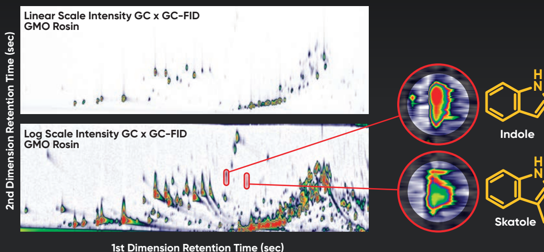
Figure 6. Two-dimensional chromatograms, adjusted with varying intensity scales, illustrate how minor compounds like Indole and Skatole can be easily overlooked.
