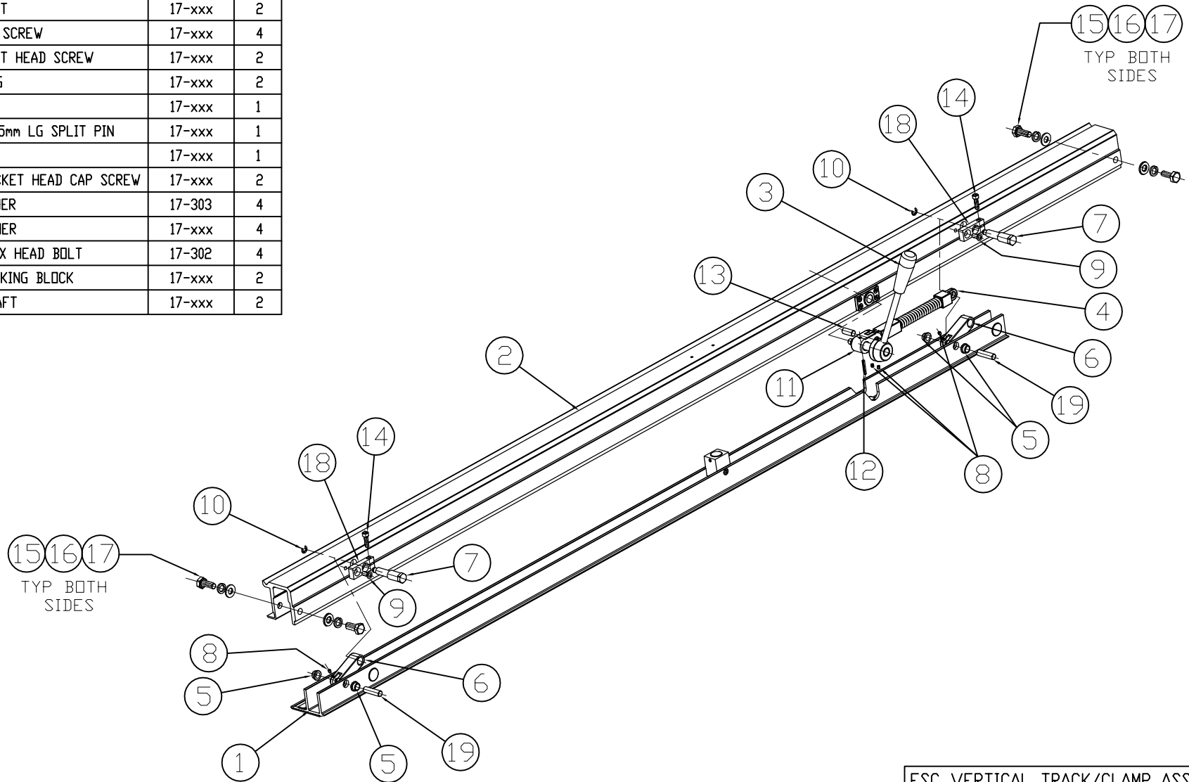
FSC VERTICAL TRACK/CLAMP ASSEMBLY
