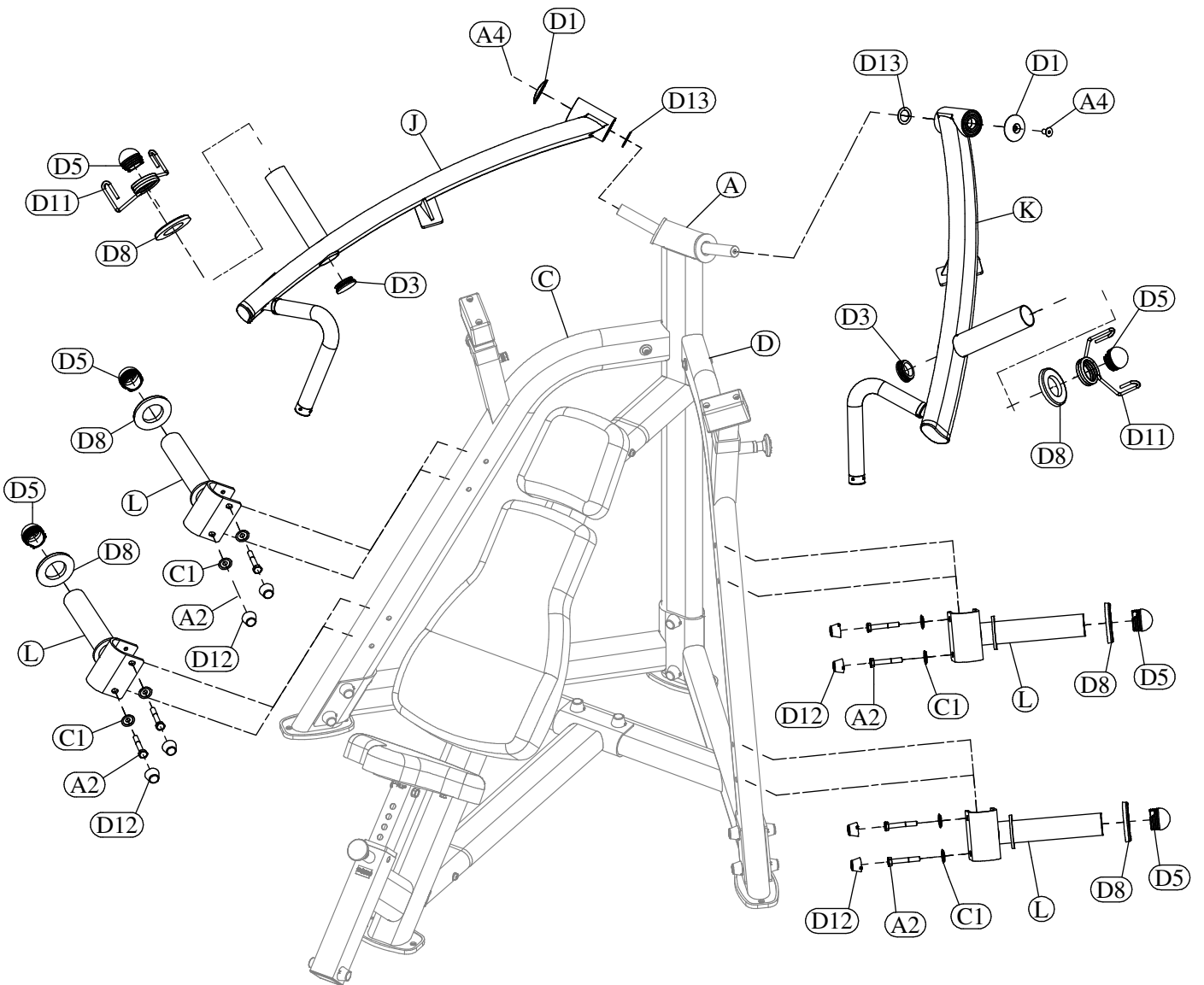
Above shows STEP 5 assembled and completed
