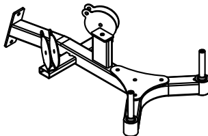
PART D-FRAME D, 1PCS.
