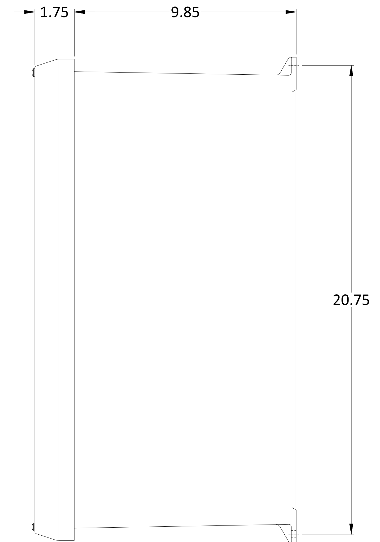
SIDE VIEW
