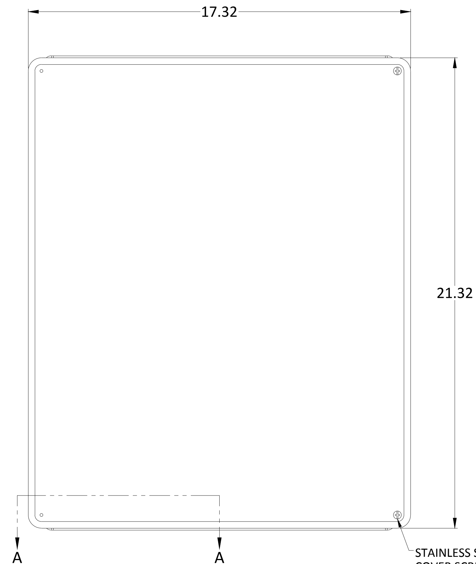
END VIEW
