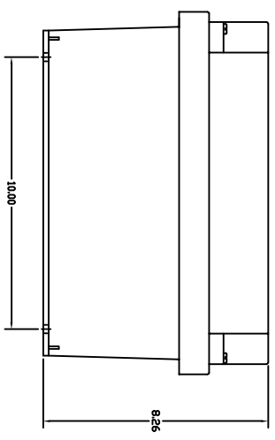
END VIEW
