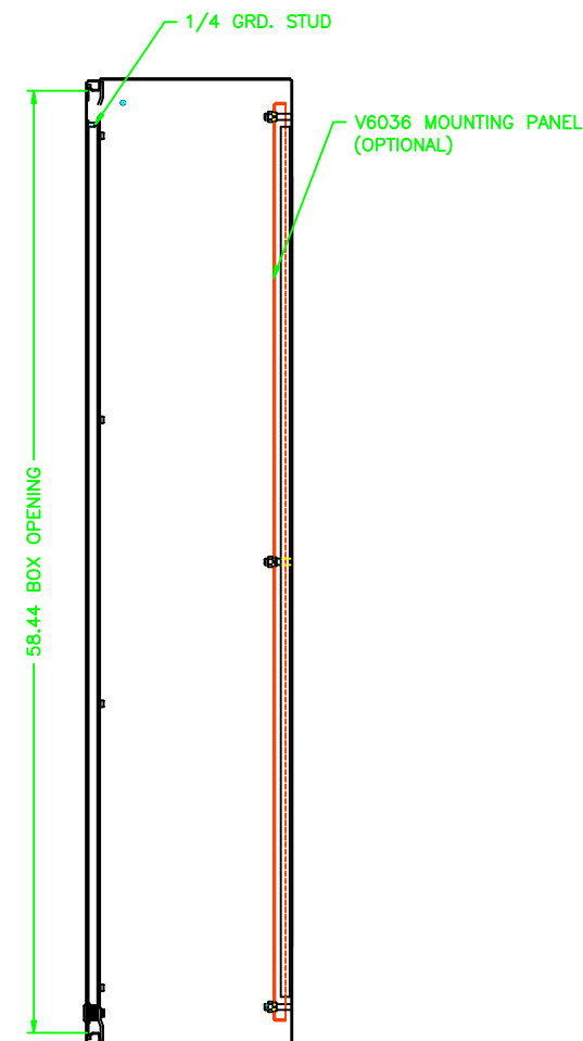
SECTION C-C
