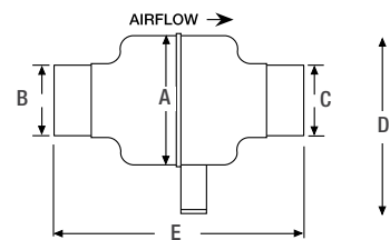
Dimensions - SF200
