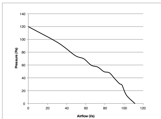
Performance - SF150
