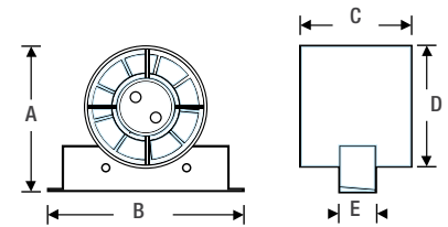
Dimensions - SF100/SF125/150
