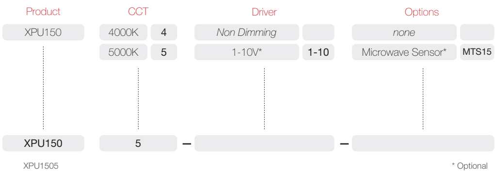
Optional microwave motion sensor Part: MTS15
