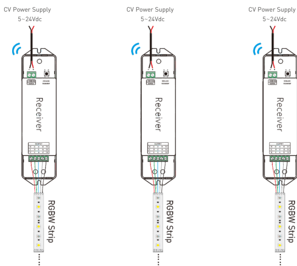
Sample wiring diagram
