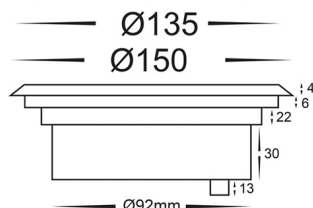
Cutout without Canister
