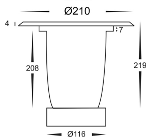
Cutout without Canister Ø182
