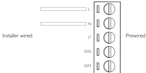
Figure 6: Inverter standard wiring diagram
