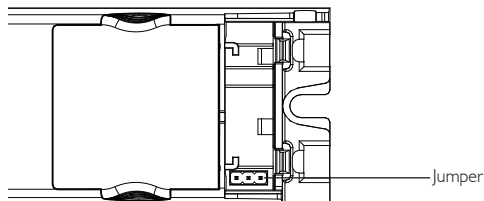
Figure 12: Maintained/non-maintained jumper
