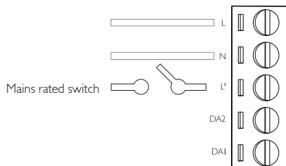
Figure 8: Inverter switch wiring diagram
