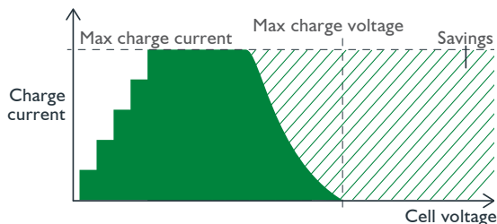
Figure 3: Smart charge rate
