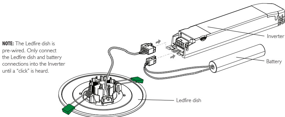
Figure 1: Ledfire assembly and ceiling installation
