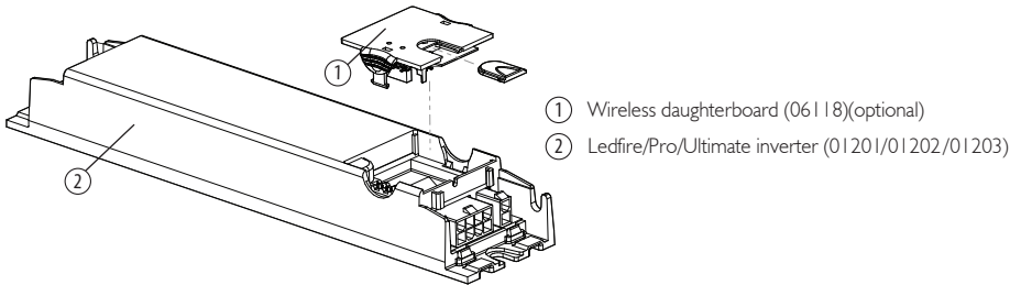
Figure 4: Daughterboard assembly diagram
