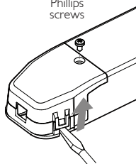
Figure 11: Changing the cable set
