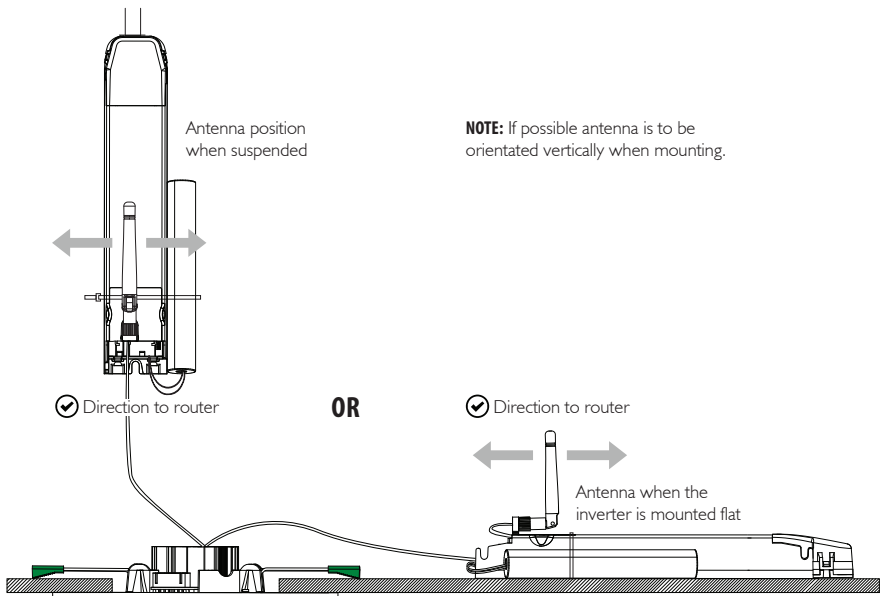
Figure 5: Mounting position of the inverter antenna
