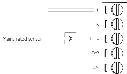
Figure 9: Inverter sensor wiring diagram
