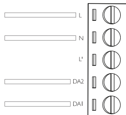
Figure 7: Inverter DALI wiring diagram
