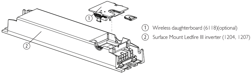
Figure 7: Daughterboard assembly diagram
