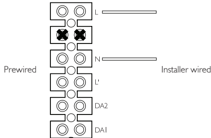
Figure 8: Inverter standard wiring diagram
