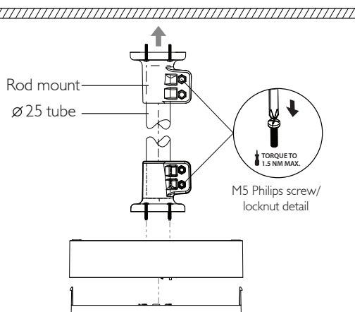
Figure 3: Rod mount installation
