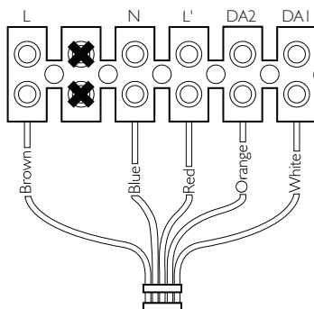
Figure 4: Wiring schematic
