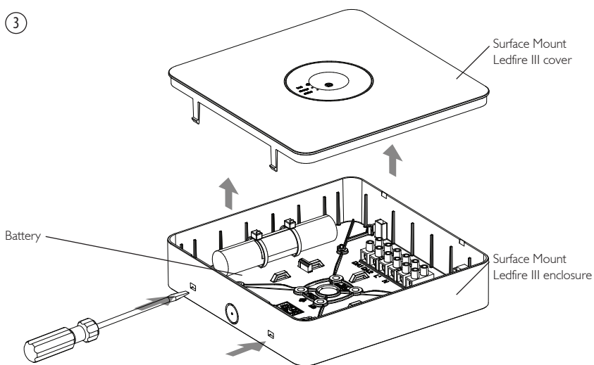
Figure 1 : Surface Mount Ledfire III disassembly and installation
