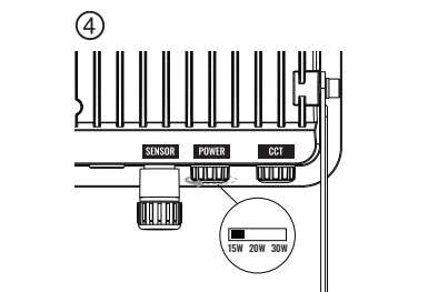
Adjust power on switch (30W model only)
