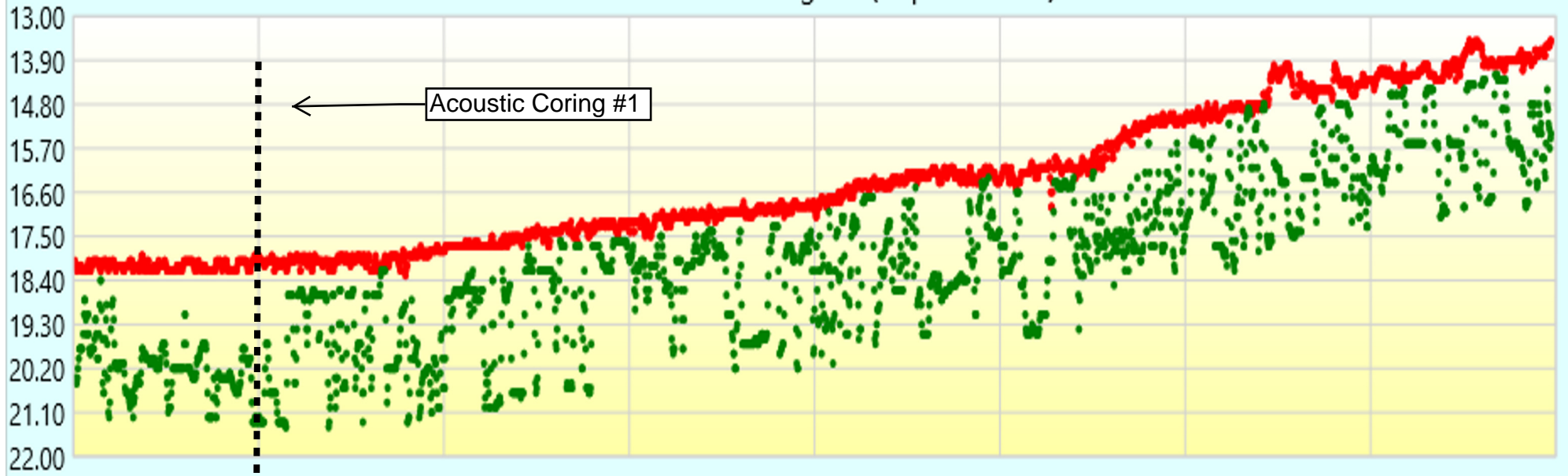
SNDG00001 - Echogram (Depth vs Time)
