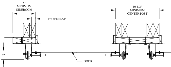
COMMERCIAL 2" CONTINUOUS ANGLE MOUNT TO WOOD JAMB DETAIL
