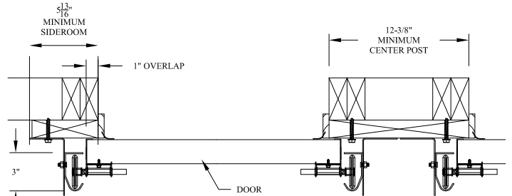
COMMERCIAL 3" TAPERED CONTINUOUS ANGLE MOUNT TO WOOD JAMB DETAIL
