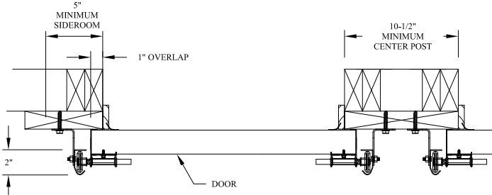
COMMERCIAL 2" BRACKET MOUNT TO WOOD JAMB DETAIL
