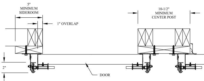
COMMERCIAL 2" REVERSE ANGLE MOUNT WITH JAMB BRACKET ATTACHMENT TO WOOD JAMB DETAIL
