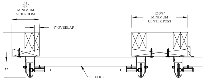
COMMERCIAL 3" REVERSE ANGLE MOUNT WITH JAMB BRACKET ATTACHMENT TO WOOD JAMB DETAIL
