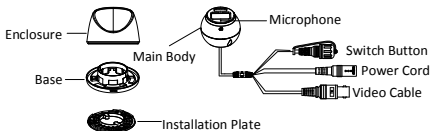
Figure 1-5 Overview of Type III Camera (DF3T series)
