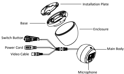
Figure 1-9 Overview of Type V Camera (DF3T Series)
