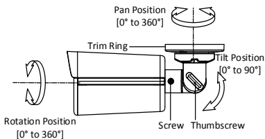
Figure 2-2 3-Axis Adjustment
