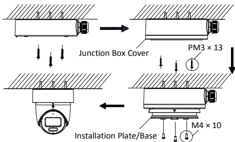
Figure 2-11 Fix the Camera to the Junction Box
