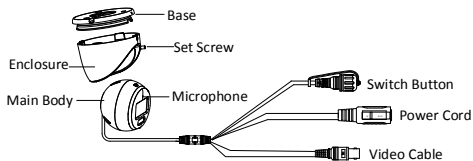
Figure 1-7 Overview of Type IV Camera (DF3T Series)
