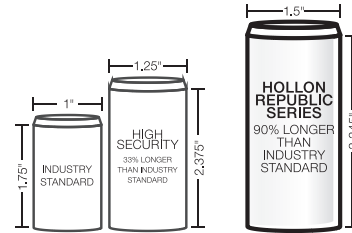
COMPARE INDUSTRY AND HOLLON BOLT SIZES
