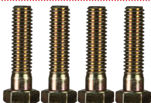
(FOUR) HEX BOLT 3/8"-16x2-1/4"
