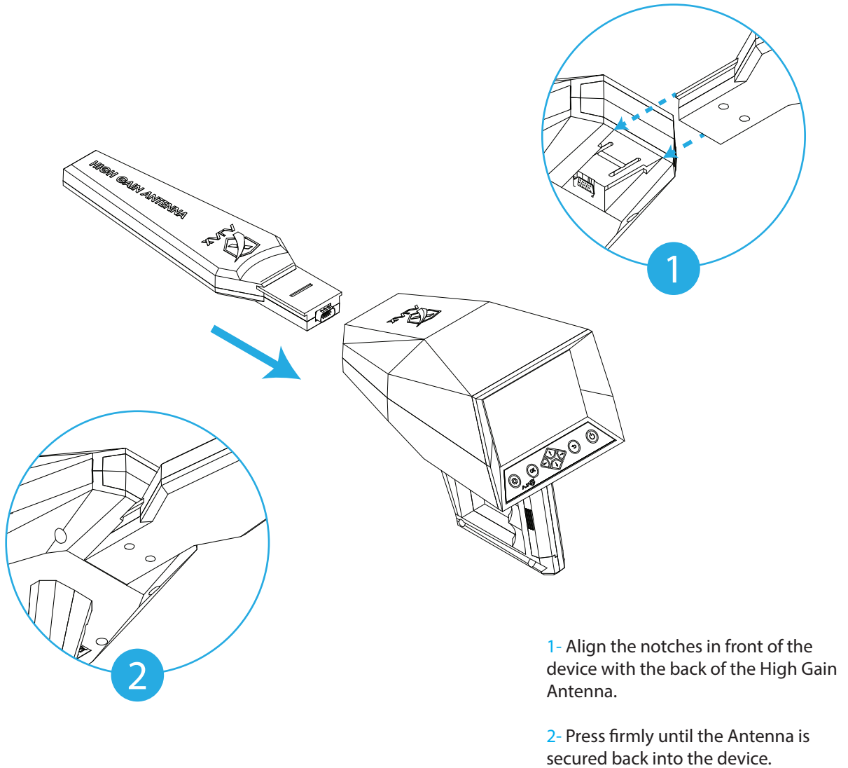
figure 5 -High Gain Antenna Assembly
