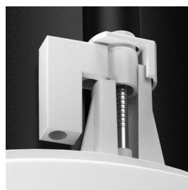
Quick Lock Mounting Rotating locking lugs for secure rattle free mounting
