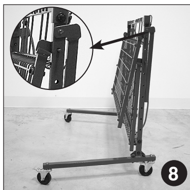
8 Nesting instructions Using the dedicated nesting holes, store one shelf on back of cart and one on front (as shown).
