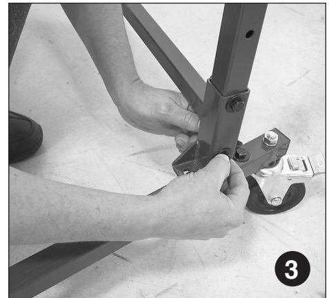
3 Slide side rail tube into lower base support. Insert bolts. Note: do not tighten bolts until frame is completed.
