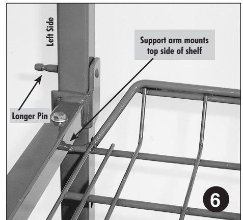
6 Shelf assembly Put longer pin on the left side of all shelves.
