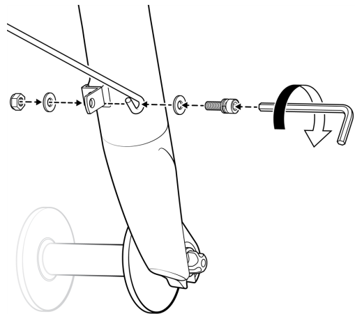
fender/mudguard mounting hardware
