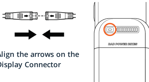
Battery button
