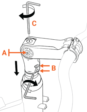
Stem/handlebar installation
