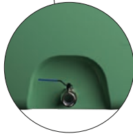
2" bottom outlet fitted with stainless steel ball valve
