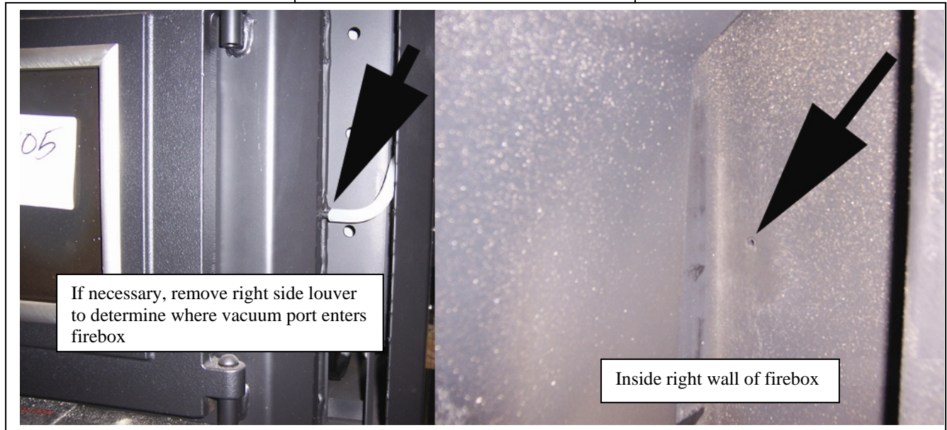
"Door Ajar" Vacuum Switch Port
