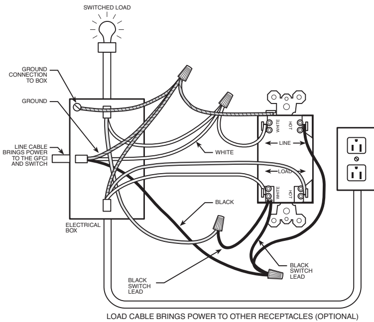
Wiring Diagram B1 (Single Switch Cat. #1595SWT)
