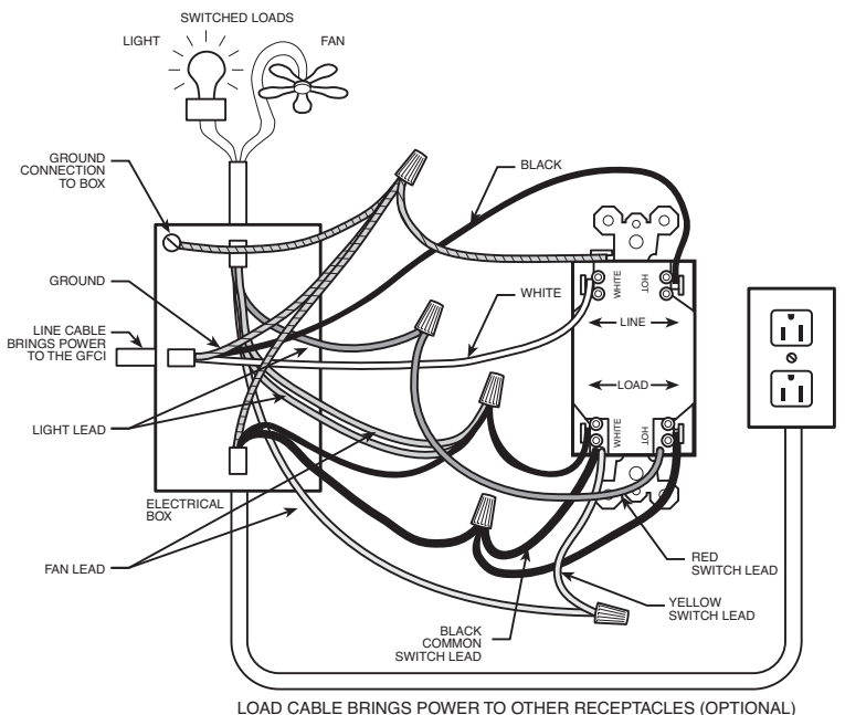
Wiring Diagram C2 (Double Switch Cat. #15952SWT)
