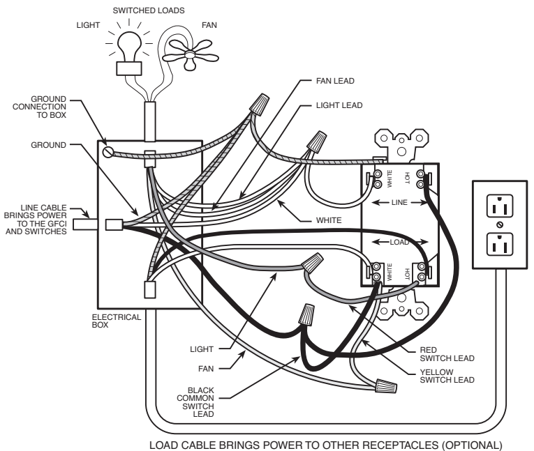
Wiring Diagram B2 (Double Switch Cat. #15952SWT)
